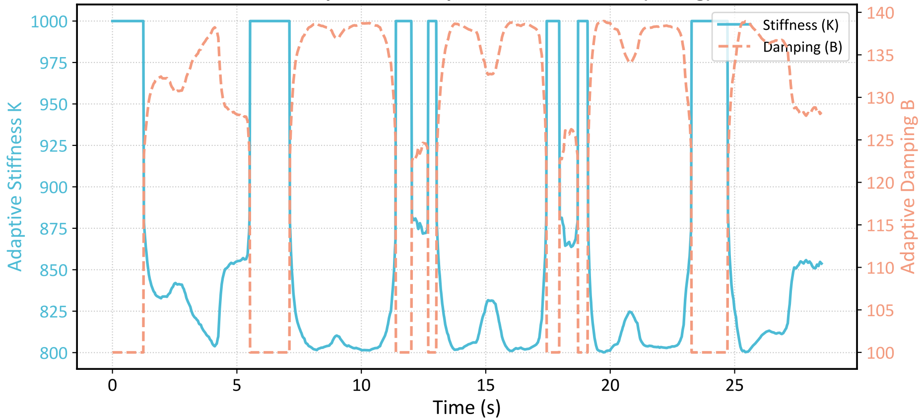
Online Adaptation of Impedance Parameters (Lifting)
